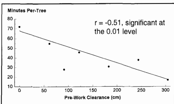
Figure 3. Relationship between proximity to the conductors and time (worker-minutes) to prune trees at utility B.
