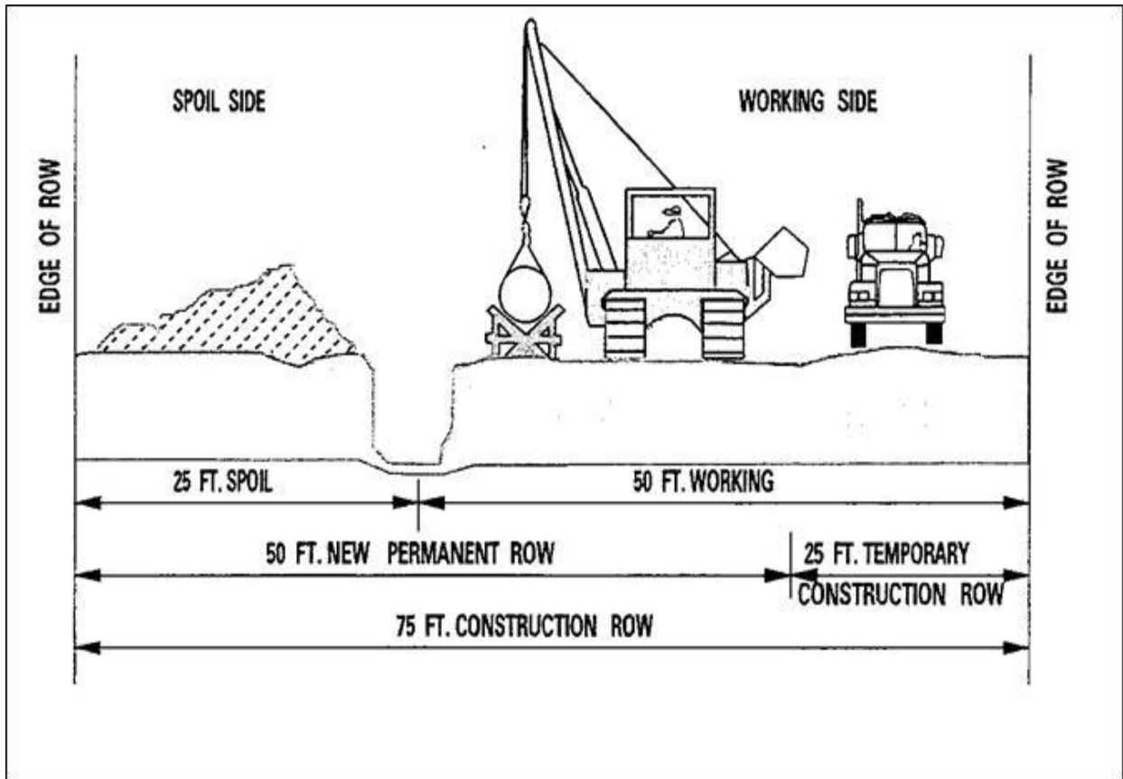
Figure 1: Typical 75-foot construction right-of-way
