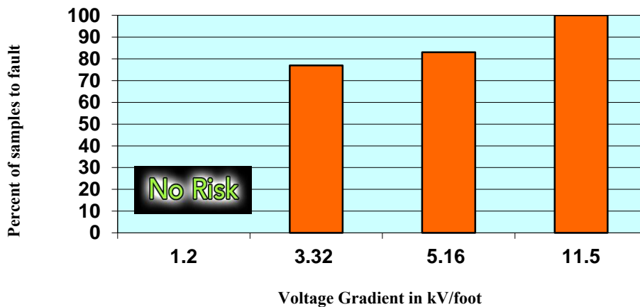
Figure 6. Influence of Voltage Gradient on Likelihood to Fault
